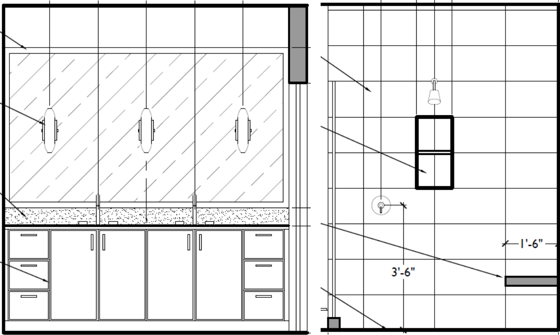
VANITY & SHOWER ELEVATION
